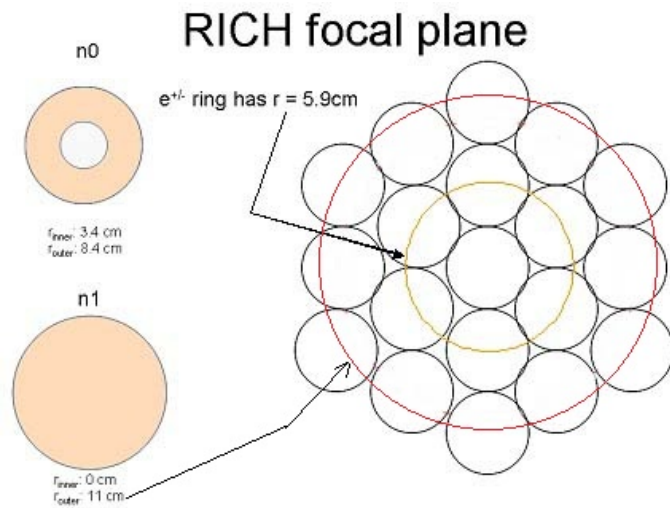
Figure 2.23: Derivation of RICH Variables.
