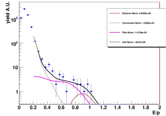
E/p (12.00-13.00)GeV p_T bin
